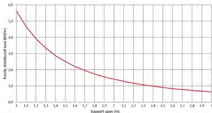
Permissible load KP 60/600 d=1,0mm (kN/m)
