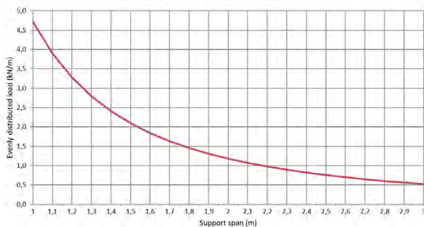
Permissible load KP 60/400 d=1,0mm (kN/m)
