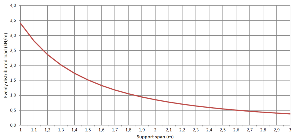
Permissible load KPK 100/100 d=0,75mm (kN/m)
