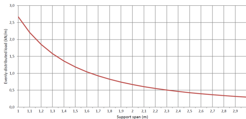
Permissible load KPK 80/100 d=0,75mm (kN/m)
