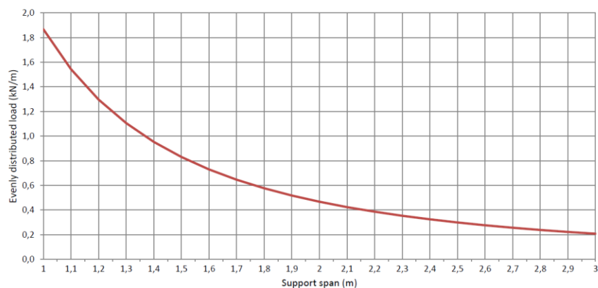
Permissible load KPK 60/200 d=0,6mm (kN/m)
