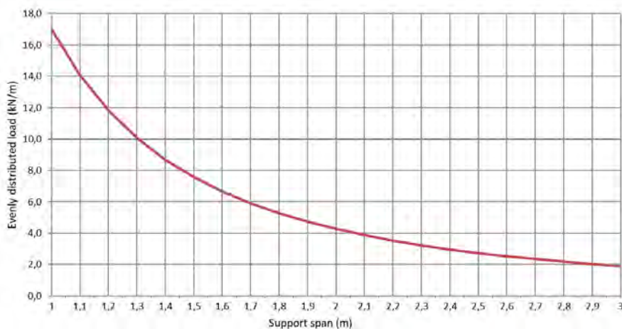
Permissible load KP 100/600 d=1,5mm (kN/m)
