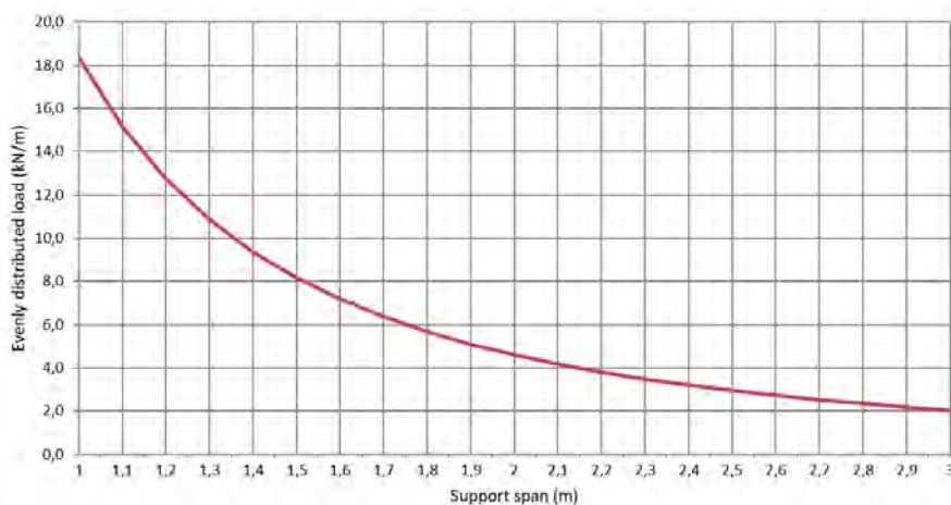
Permissible load KP 100/400 d=1,5mm (kN/m)
