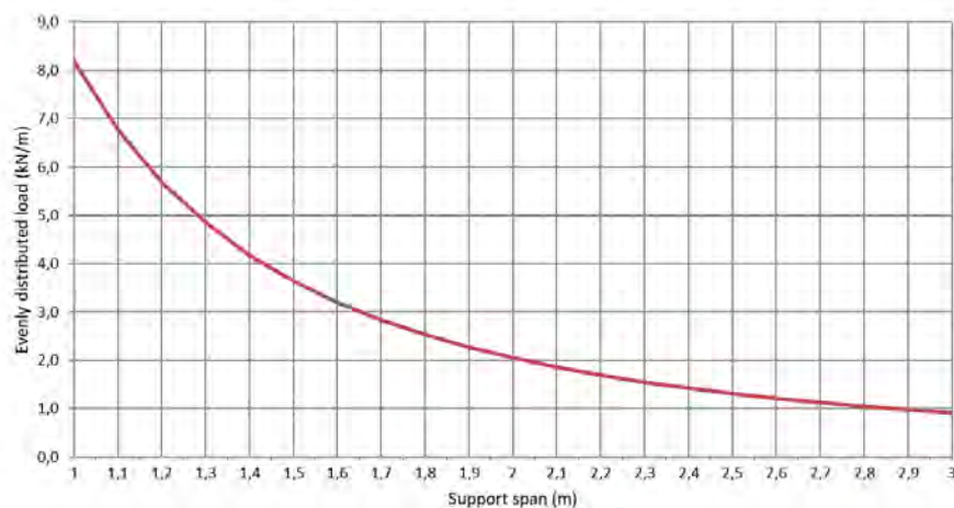
Permissible load KP 60/300 d=1,5mm (kN/m)
