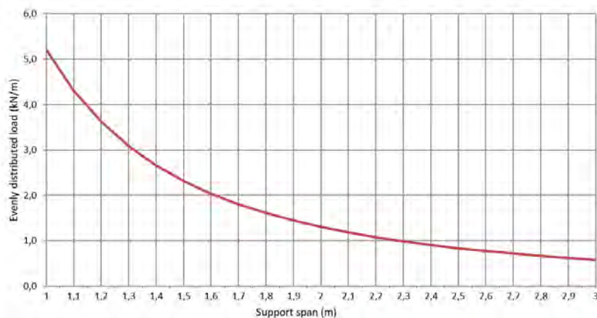
Permissible load KP 60/500 d=1,0mm (kN/m)
