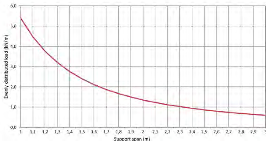
Permissible load KP 100/600 d=1,0mm (kN/m)
