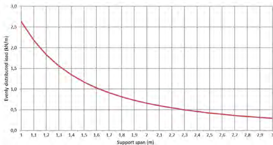
Permissible load KP 40/600 d=0,8mm (kN/m)
