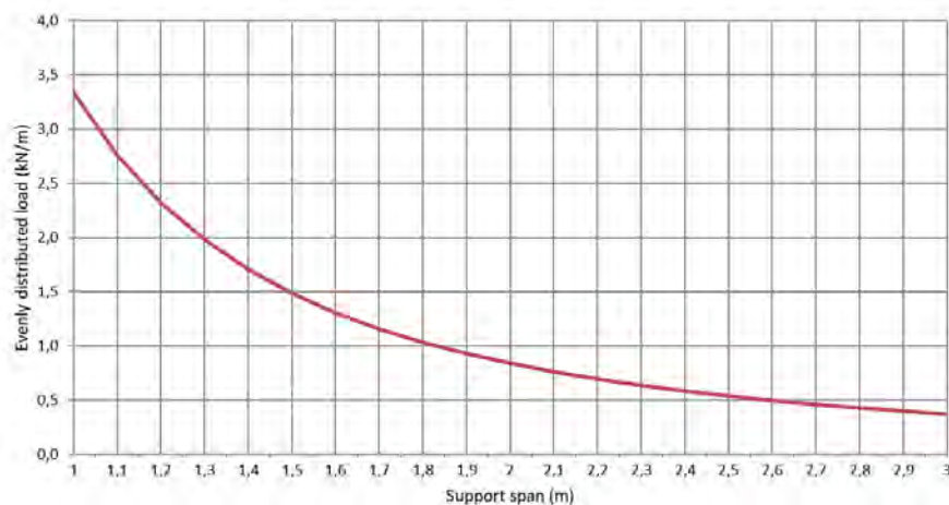
Permissible load KP 60/400 d=0,8mm (kN/m)
