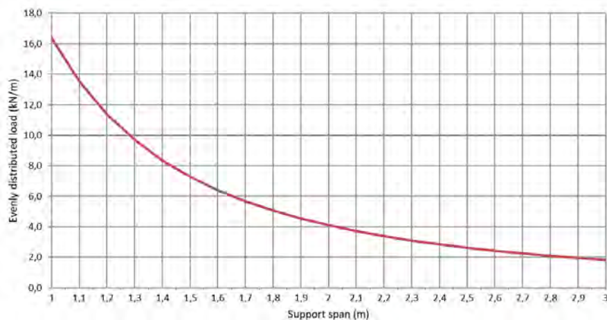
Permissible load KP 100/300 d=1,5mm (kN/m)
