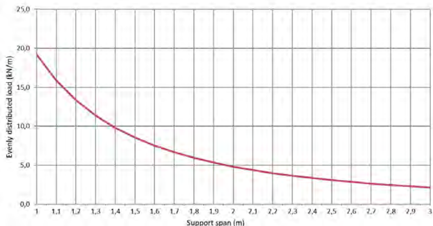
Permissible load KP 100/500 d=1,5mm (kN/m)
