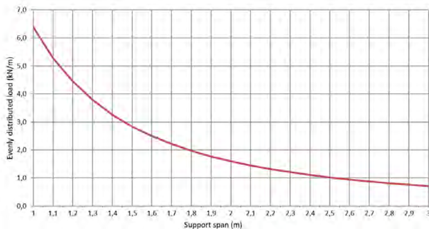
Permissible load KP 100/500 d=1,0mm (kN/m)
