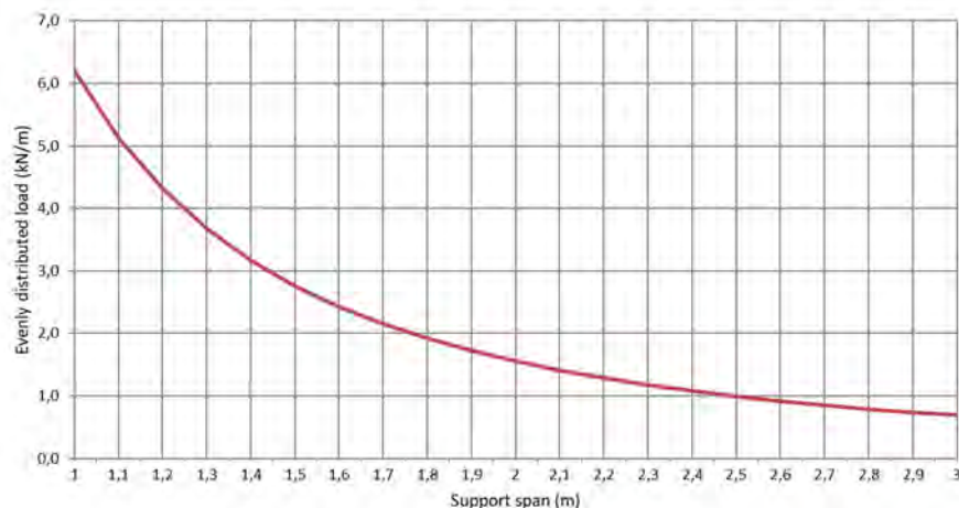
Permissible load KL 60/600 d=1,0mm (kN/m)
