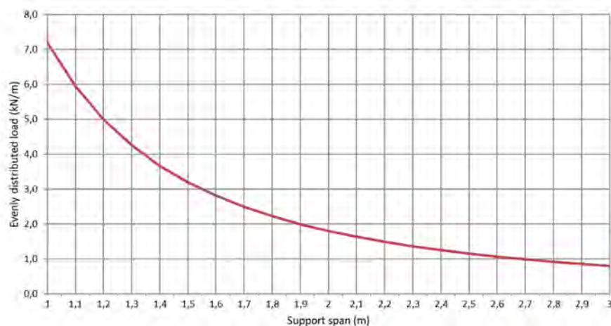
Permissible load KL 60/400 d=1,0mm (kN/m)
