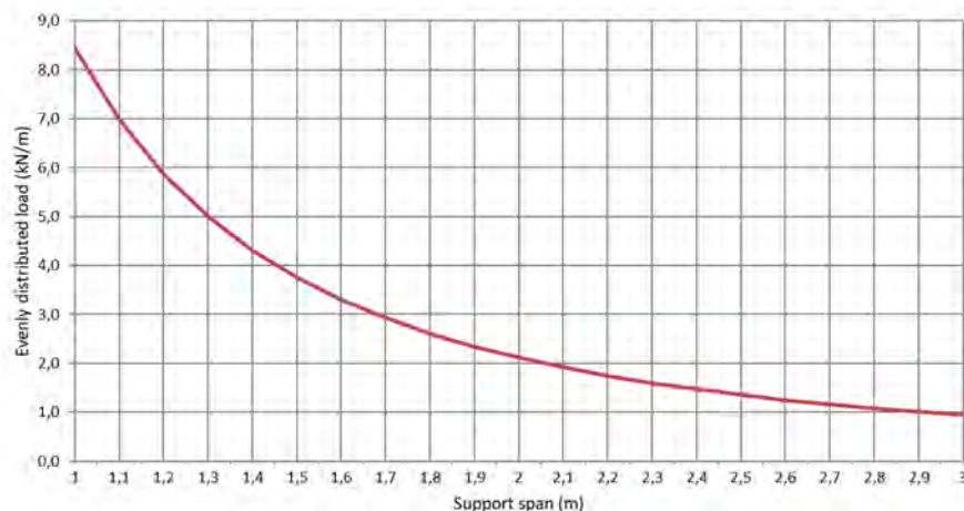
Permissible load KL 100/400 d=1,0mm (kN/m)
