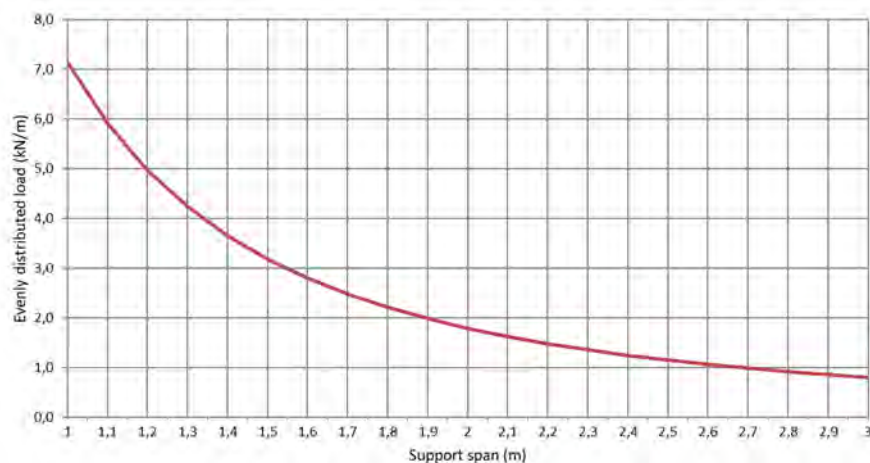
Permissible load KL 100/300 d=1,0mm (kN/m)
