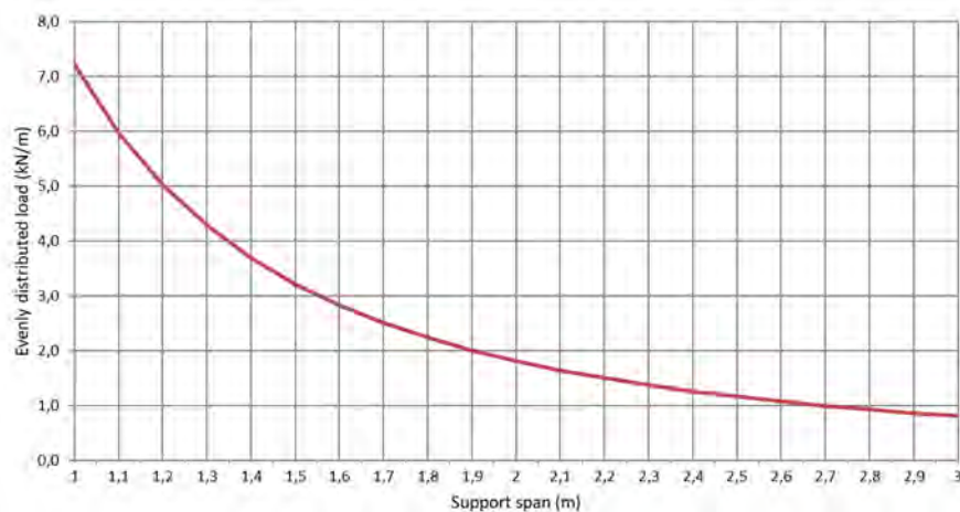
Permissible load KL 100/600 d=1,0mm (kN/m)
