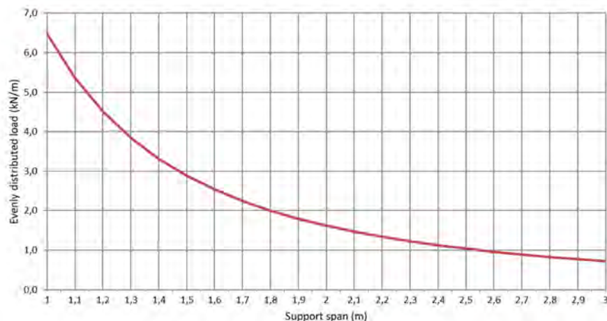
Permissible load KL 60/300 d=1,0mm (kN/m)
