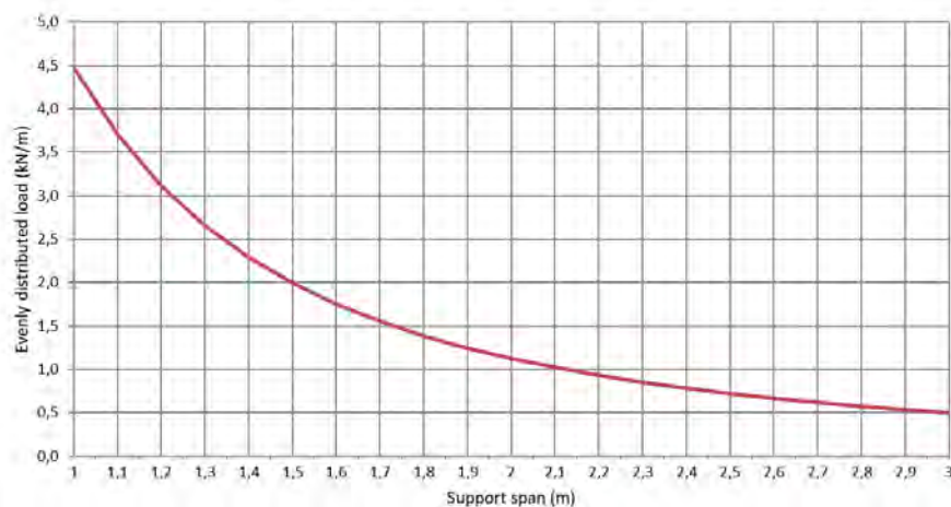
Permissible load KP 60/300 d=1,0mm (kN/m)
