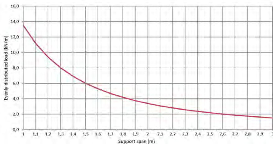
Permissible load KP 60/600 d=1,5mm (kN/m)
