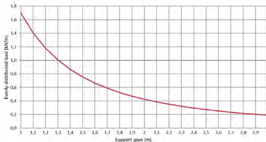
Permissible load KPA 60/500 d=1,0mm (kN/m)
