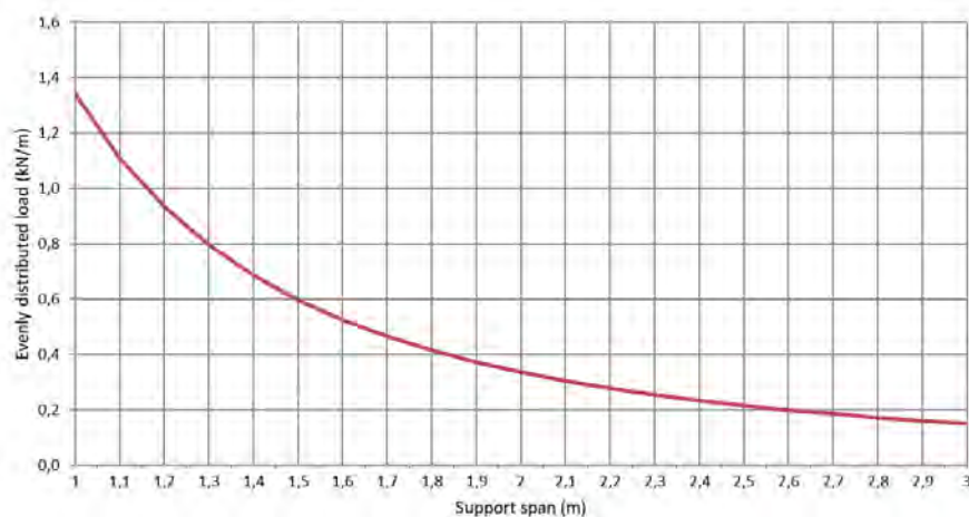
Permissible load KPA 60/100 d=1,0mm (kN/m)
