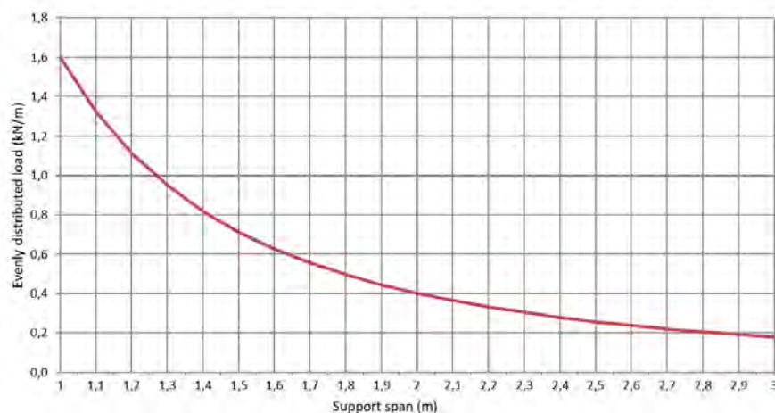
Permissible load KPA 60/600 d=1,0mm (kN/m)
