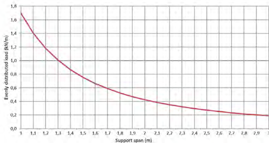
Permissible load KPA 60/500 d=1,0mm (kN/m)
