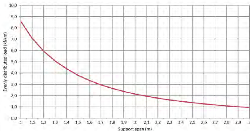
Permissible load KLA 100/100 d=2,0mm (kN/m)
